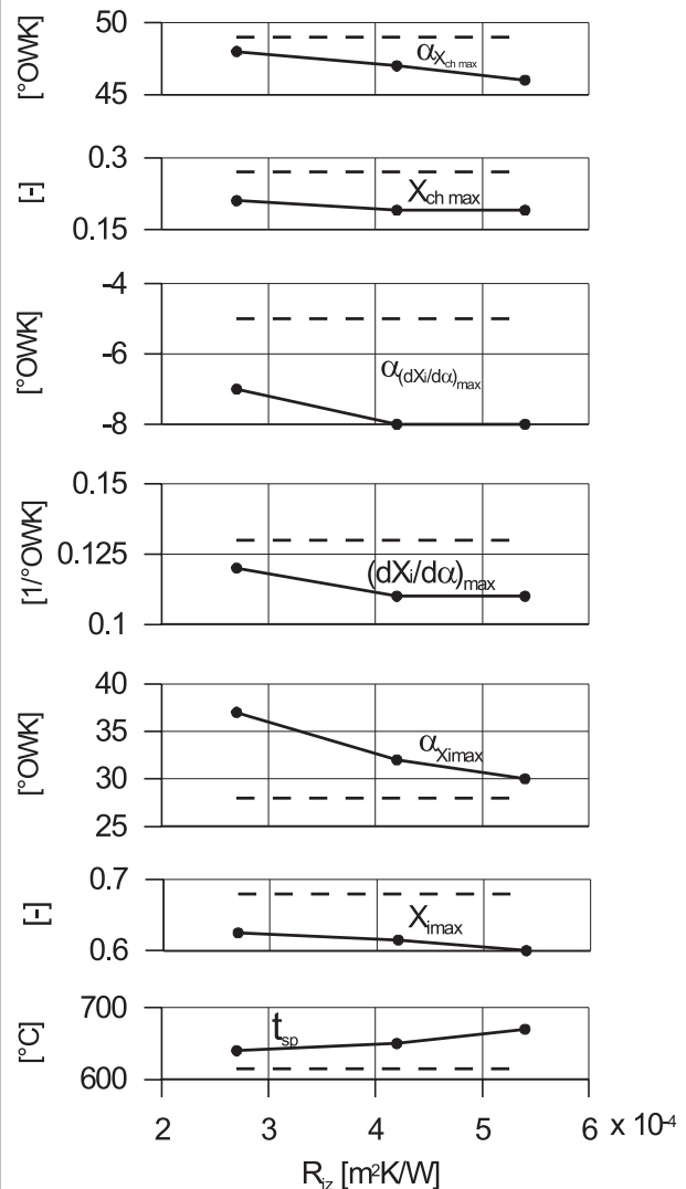
Fig. 2. Influence of heat resistance of insulating coatings on piston heads on combustion indicators; n = 2200 \text{ rpm} , p_e = 0.6 \text{ MPa} . Broken line - values for piston without coating.
