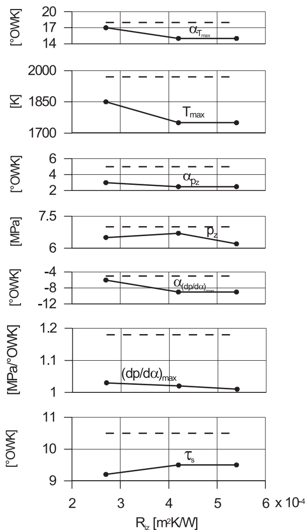
Fig. 1. Influence of heat resistance of insulating coatings on piston heads on combustion indicators; n = 2200 \text{ rpm} , p_e = 0.6 \text{ MPa} . Broken line - values for piston without coating.
