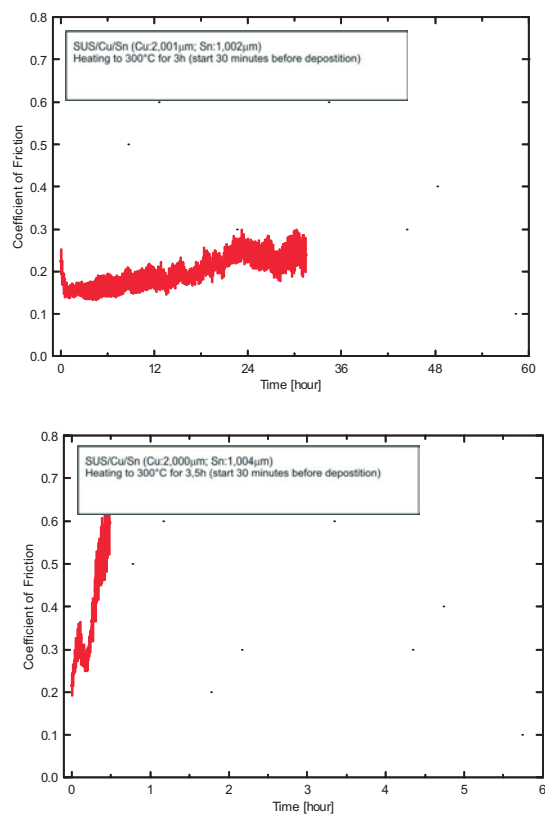
Fig. 7. Friction tests of heated specimens: Cu being 2.0 \mu\text{m} and Sn being 1.0 \mu\text{m} thick
