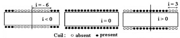
Fig. 4. Distribution of the turns \rho(x) on the core, for different values of index i .
