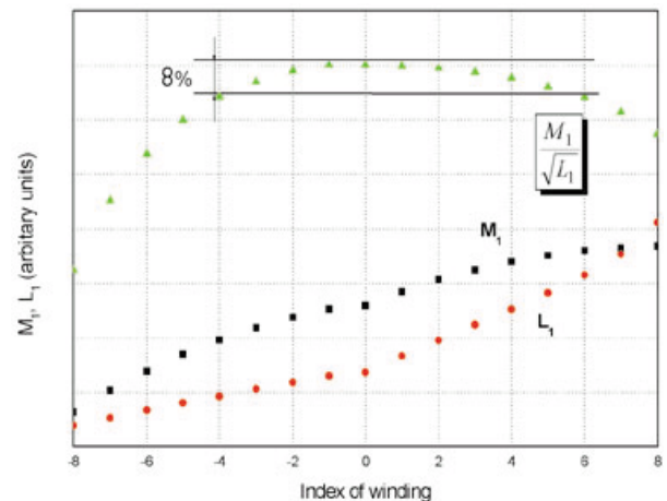
Fig. 5. Physical properties for special windings. Self-inductance L_1 and mutual M_1 inductance are standardized per 1 turn. Signal sensitivity k_S is proportional to M_1/\sqrt{L_1} .
