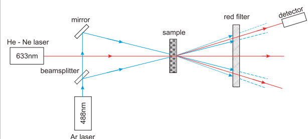
Fig. 1 Experimental set up for self-diffraction investigation.
