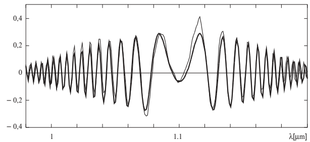
Fig. 3 Comparison of measured spectral dependence and dependence calculated assuming linear dispersion of the refractive indices
