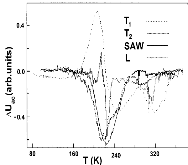
Fig. 1 A-DLTS spectra of Cr-doped GaAs obtained for various generated acoustic waves
