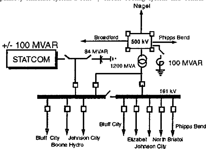
Obr. 10. Schéma zapojenia elektrickej stanice Sullivan Fig. 10. Scheme of connection of electric station Sullivan
