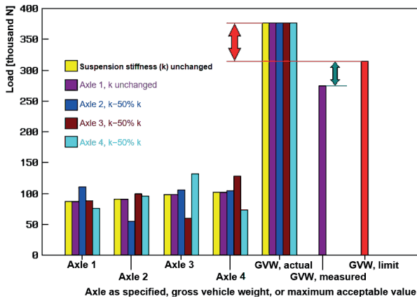
Figure 12 Calculation results for the example four-axle motor truck overloaded by 20%, compared to the maximum acceptable load values. Loads on individual axles (“Axle 1”, “Axle 2”, “Axle 3”, “Axle 4”), actual gross vehicle weight (“GVW, actual”), gross vehicle weight limit (“GVW, limit”) and gross vehicle weight measurement result obtained with changing the suspension stiffness at axle 2, 3 and 4 as described (“GVW, measured”)
