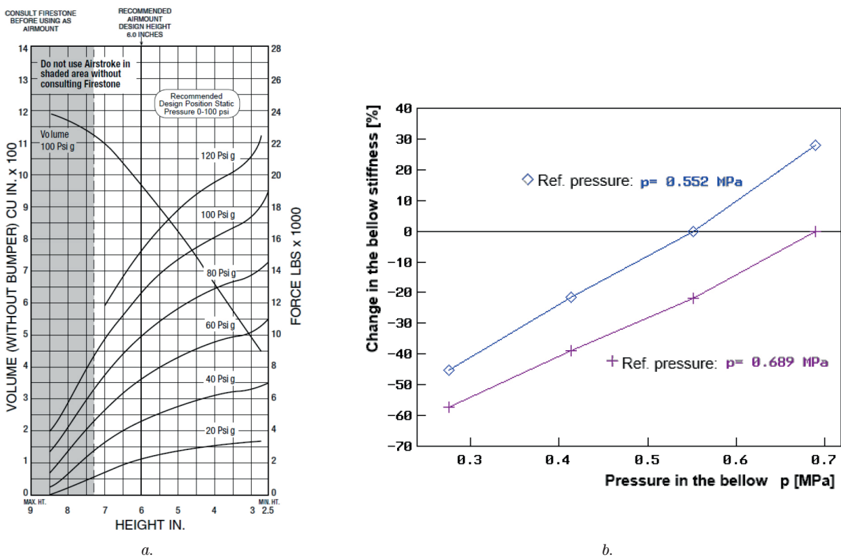
Figure 2 a. Example characteristics of the pneumatic suspension spring (air bellows) of a motor truck: force (lbs×1 000=4.54×1 000 N) vs current bellows height (in = 0.0254 m) for various constant values of bellows inflation pressure (above atmospheric, e.g. 100 psig=0.689 MPa) [25], b. Relative changes in the air bellows stiffness for two different reference pressure values (0.552 MPa and 0.689 MPa in this case, as specified)
