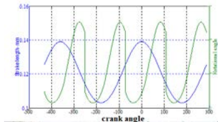
Figure 12 Variations of the rotation motion of a skirt (Case 1)
