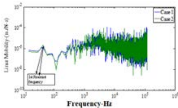
Figure 10 Variations of the piston mobility (2000 rpm)
