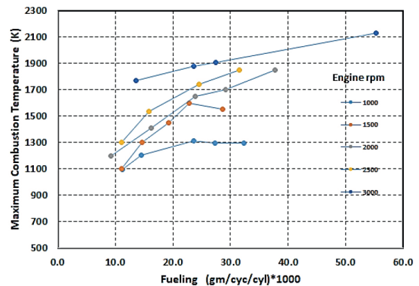
Figure 8 Maximum calculated combustion temperature
