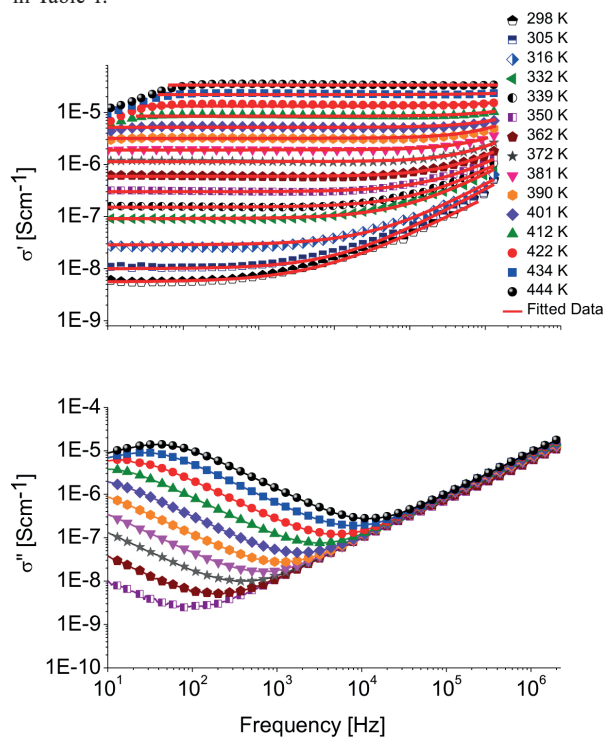
Fig. 1 Frequency dependence of real and imaginary parts of ac conductivity for glass 50\text{Li}_2\text{O} \cdot x\text{B}_2\text{O}_3 \cdot (50-x)\text{P}_2\text{O}_5 ( x = 5 mol%). Red lines represent theoretical fit accordance with Equation 2
