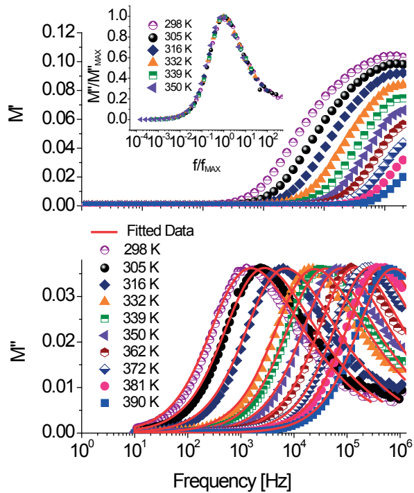
Fig. 4 Imaginary and real representation of frequency dependent modulus; red lines represent the fitted data with KWW function
