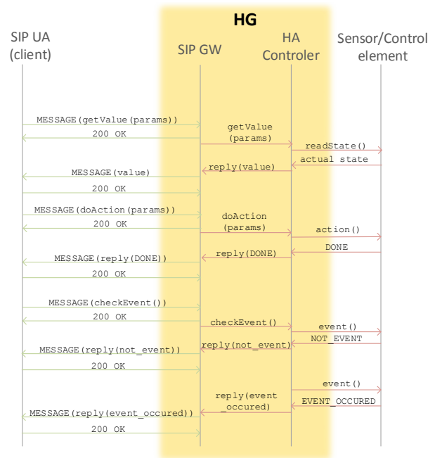
Fig. 5 Message-only model
