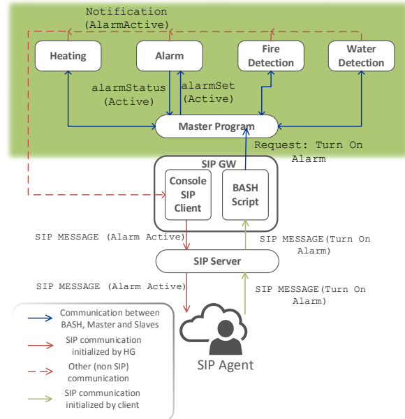
Fig. 7 Communication model of HA controller parts
