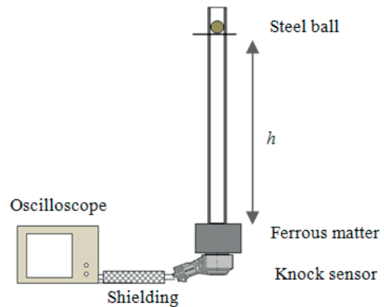
Figure 5 Testing device
