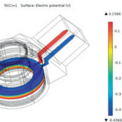
Figure 10 Output potentials of sensor with 1N of force affecting on piezoelectric element
