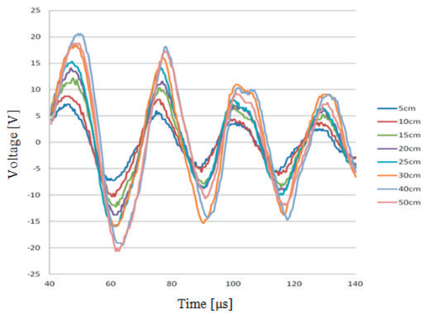
Figure 6 Output voltage of the sensor
