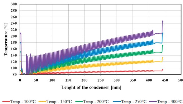
Fig. 6 Temperature dependence over the length of the condenser - Mass flow 0.03 \text{ kg.s}^{-1}
