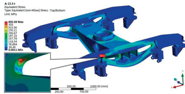
Figure 6 Results of the strength analysis for the 4 th load case
