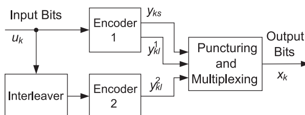
Fig. 1 Turbo encoder block diagram
