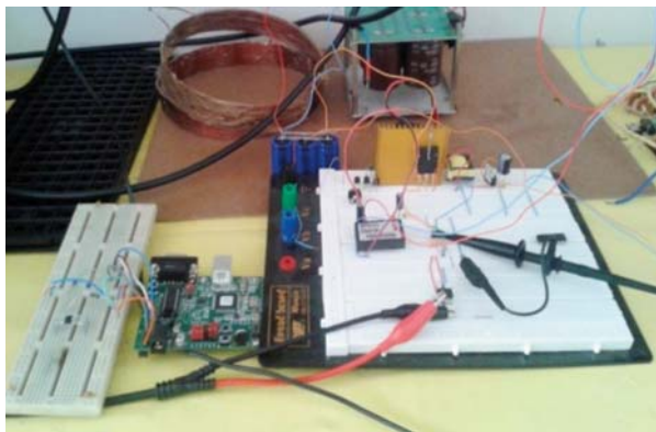
Fig. 5 Experimental set-up of proposed bidirectional step-up/step-down converter
