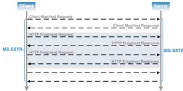
Fig. 10 MS-SSTR Communication [19]
