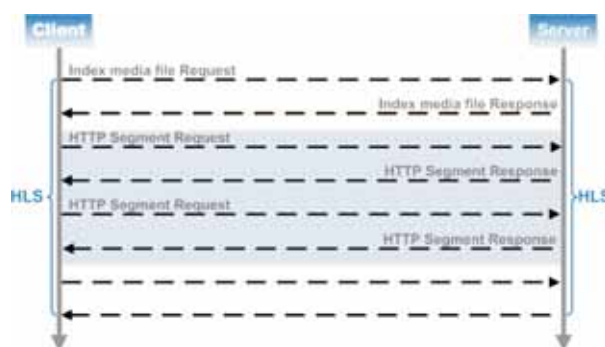
Fig. 8 HLS Communication [22]
