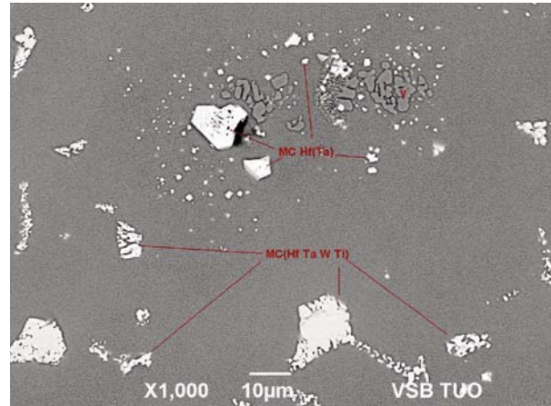
Fig. 8 Microstructure-sample 15MAW - disintegrating primary carbides (BEC)
