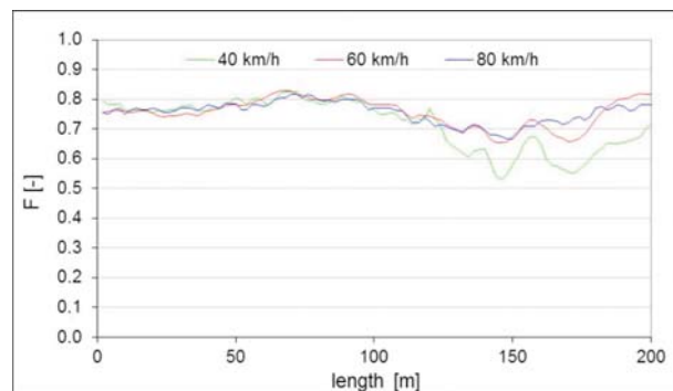
Fig. 1 Measured friction coefficient at different test speeds
