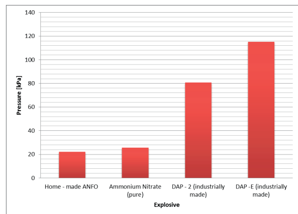
Figure 6 Maximum pressure of homemade and industrially made ANFO explosives
