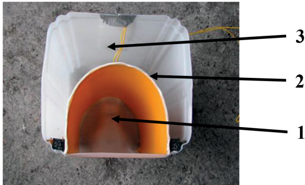
Figure 15 Body of cumulative shaped explosive
