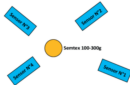
Figure 14 Disposition of blast sensors used in field test
