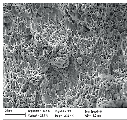
Figure 10 Dimple morphology of woody fracture
