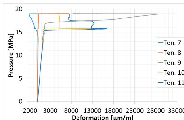
Figure 8 Dependency of pressure on deformation of the patch B
