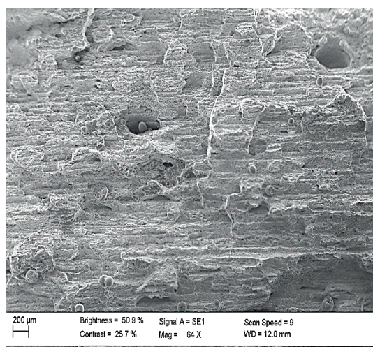
Figure 9 Woody fracture
