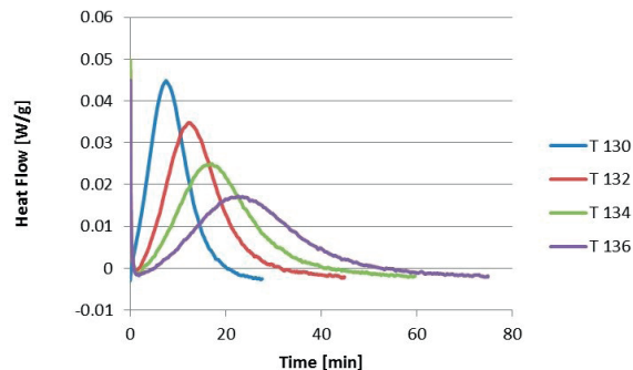
Figure 2 Heat-flow versus time during isothermal crystallization
