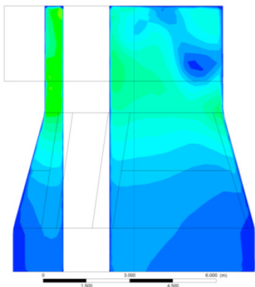
Fig. 9 Velocity field in vertical section to flue gas removal unit
