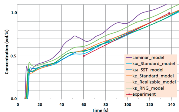
Fig. 6 Dependence of concentration change on response time of the sensor No. 2 [5]
