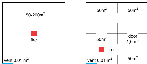
Fig.1 Geometric layout of simulated compartments (undivided left / divided right)
