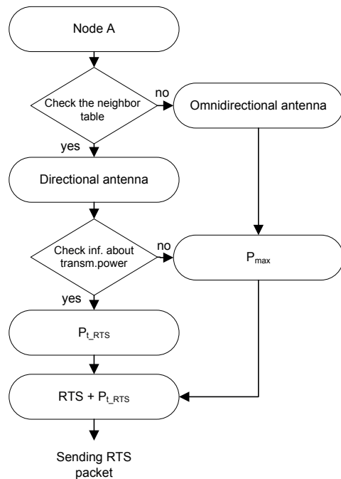
Fig. 2 Sending RTS packet
