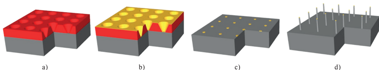
Fig. 2. Fabrication process for organized growth of NWs using NSOM lithography: a) structure patterning in photoresist layer, b) Au coating by evaporation, c) lift-off, creation of organized Au seeds and d) NWs growth by VLS technique.
