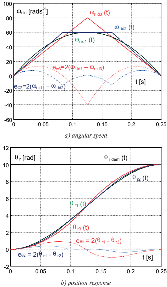
Fig. 7 Ideal state-variables for energy optimal and near-energy optimal control
