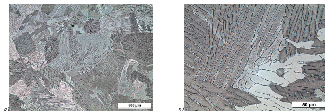
Figure 5 Ti6Al4V HT 1200 °C, a) polyhedral grains, b) coarse lamellas of \alpha+\beta phase, etch. 10% HF
