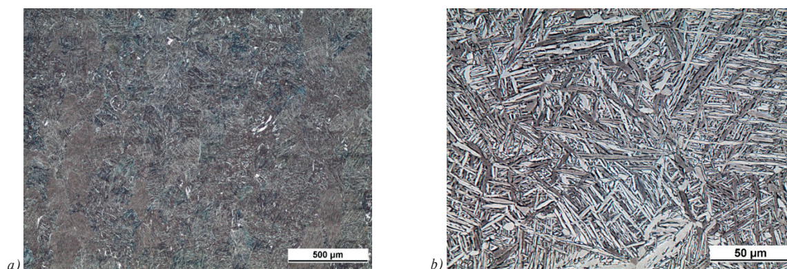
Figure 4 Ti6Al4V HT 900 °C a) columnar grains, b) coarse needles, etchant 10% HF
