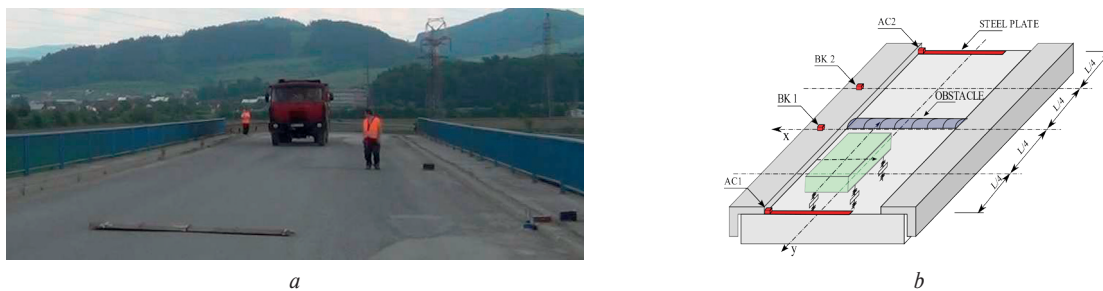
Figure 5 Situation on the bridge by the dynamic measurement, a - situation on the bridge and lorry, b - positions of the sensors
