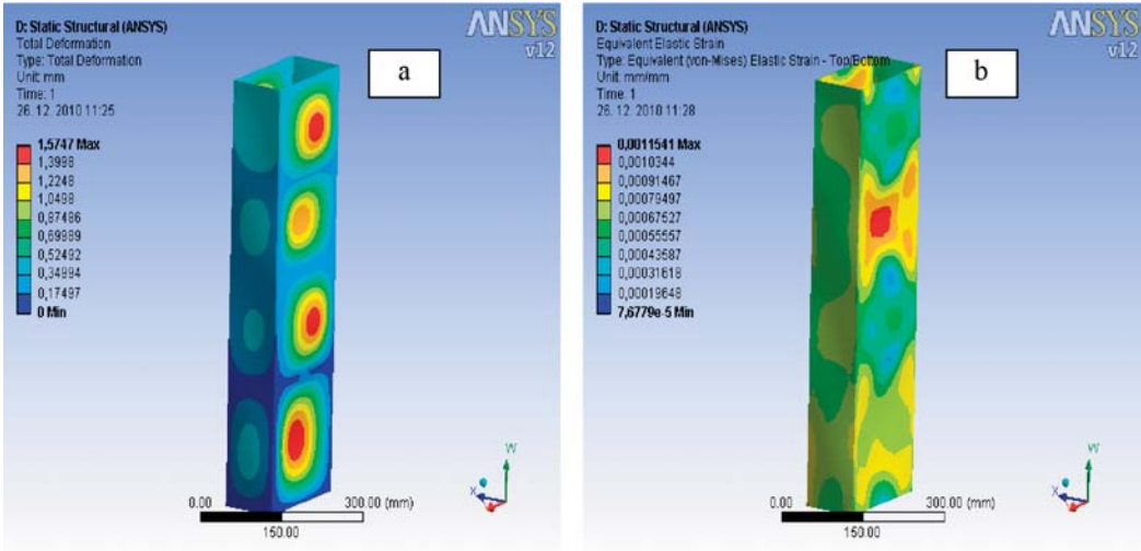
Fig. 4 Final deformation (a) and equivalent elastic strain (b), member B22
