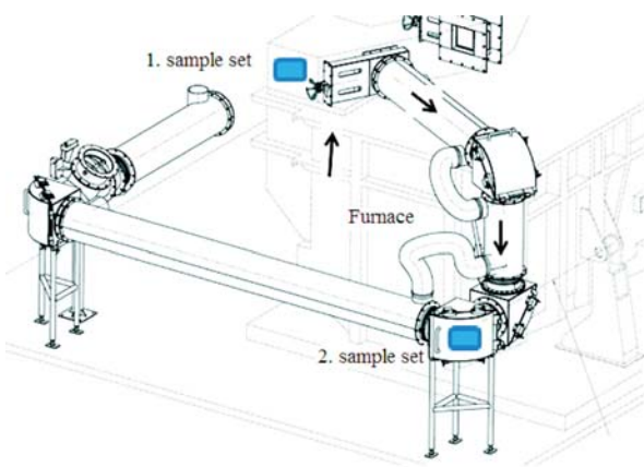
Fig. 1 Scheme of the furnace, location of samples and direction of gas flow
