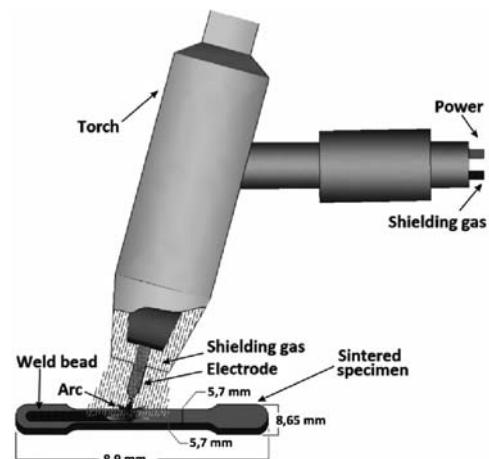
Fig. 2 Surface remelting using GTAW method
