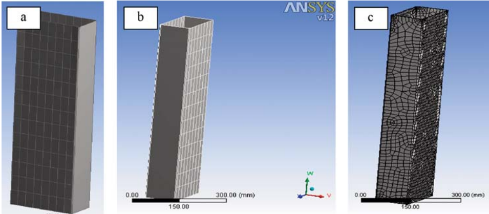
Fig. 3 Configuration of the calculation model, member B22
