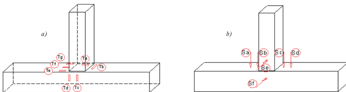
Fig. 3 Arrangement of (a) strain gauges, (b) inductive sensors and deformaters
