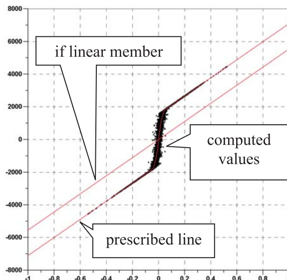
Fig. 4 A secondary suspension damper (left: given parameters, right: a comparison)
