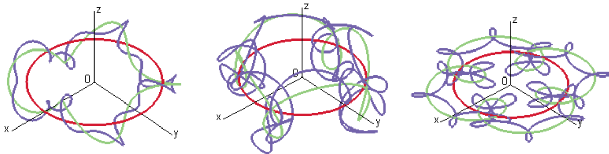
Fig. 3 Combinations of the curves k_1, k_2^t, k_3^{tt}, k_1^n, k_2^n, k_3^{nn} and k_1^b, k_2^b, k_3^{bb} .
