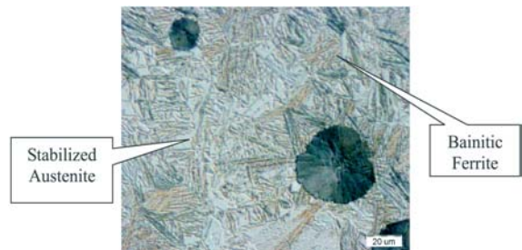
Fig. 3: The matrix microstructure of ADI for the transformation dwell of 60 minutes.
