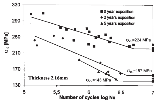
Fig. 6 Wöhler curves of the sheet 2.16 mm thick after 0 - 2 and 5-year exposition to atmospheric corrosion
