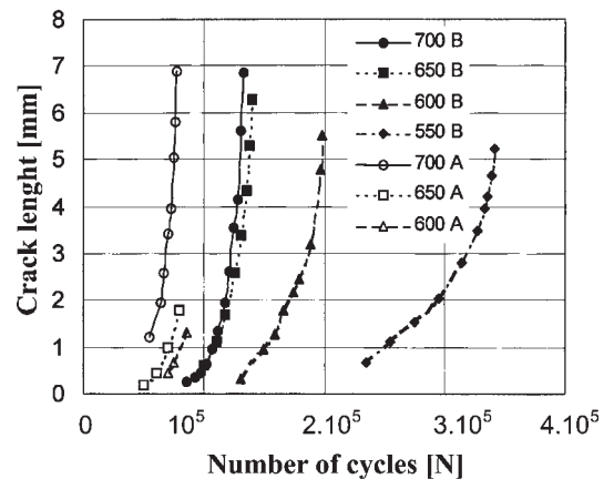
Fig. 4 Fatigue crack growth dependence on the number of cycles in E 700 TS steel at the stress of 700, 650, 600 and 550 MPa.
