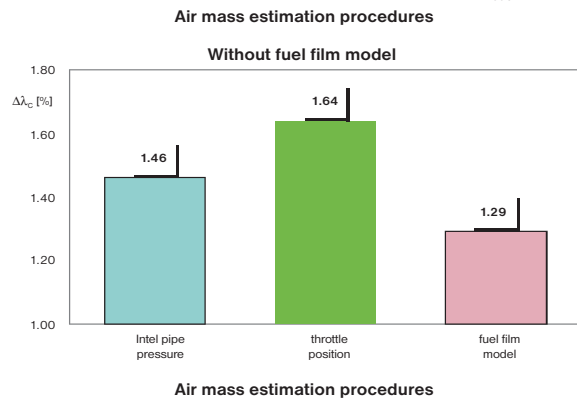
Fig. 6 Comparison of the total control error for the three methods of the cylinder air assessment and two methods including influence of the fuel film phenomena.
