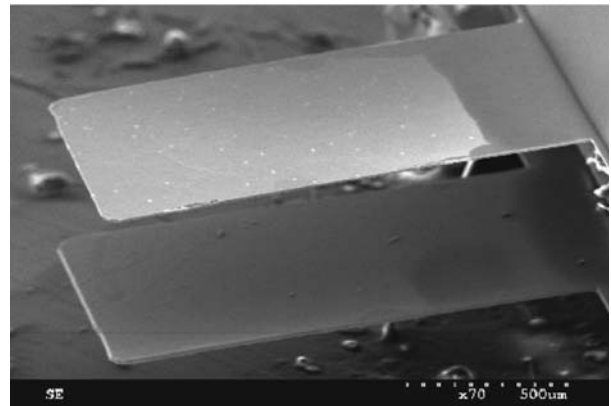
Fig. 8. Microgripper http://www.ntu.edu.sg/mpe/Research/Programmes/MEMS/Project/weimin1.html#publication
