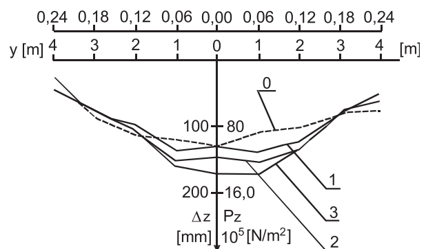
Fig. 2 Chart of vertical pressures on the soil. Sand reinforced with triple unwoven fabric Terratex 600 at changeable depth [6, 7].
