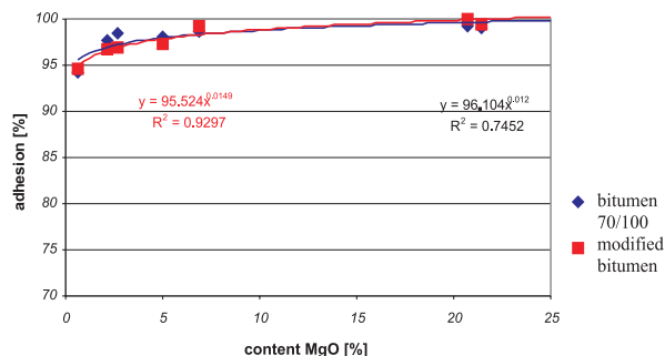
Fig. 4 The adhesion results of bitumen binder to aggregate in dependence of content MgO in aggregate
