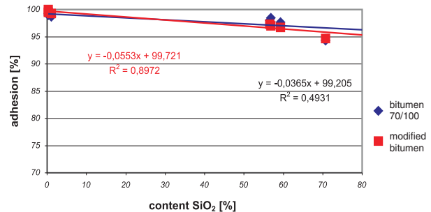
Fig. 2 The results of bitumens and aggregates adhesion
