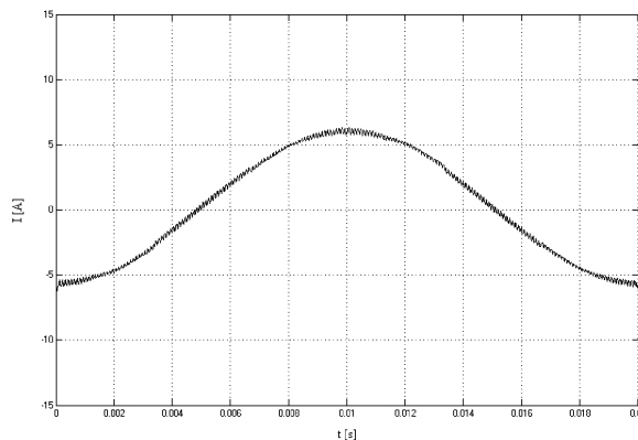
Fig. 2. Stator voltage and corresponding stator current while the motor is working in steady state ( f_s = 10 \text{ kHz} , f_{Uout} = 50 \text{ Hz} (MATLAB simulation))
