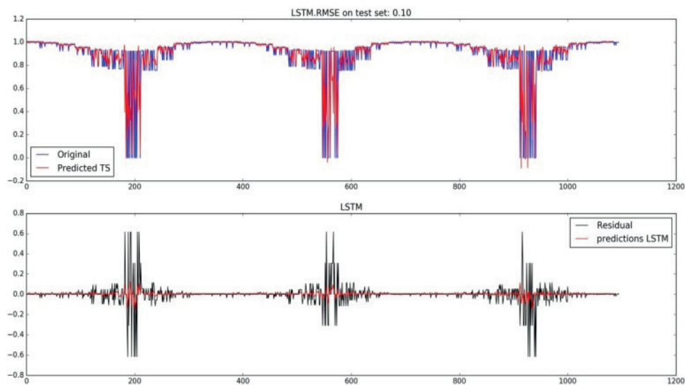
Figure 6 Description of the original time series and residues by the LSTM model
