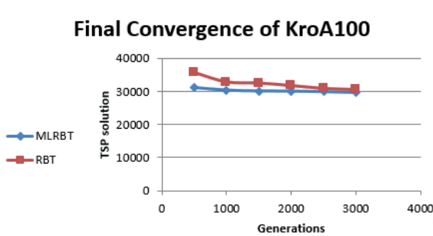
Figure 12 KroA100 - overview of performance
