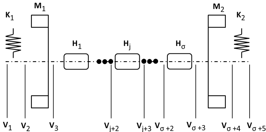
Figure 2 Model of the whole Cardan mechanism
