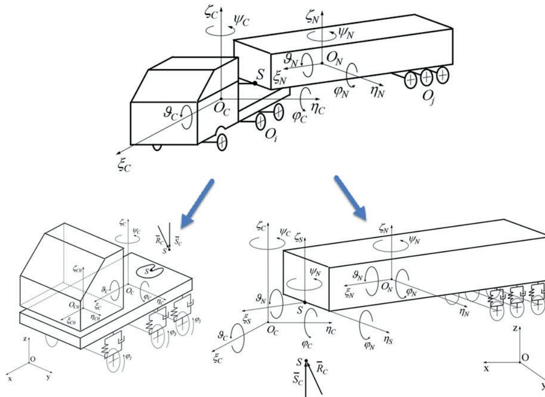
Figure 3 Model of a tractor-semitrailer unit for the simulation of the vehicle motion and dynamics, including real time simulation. 29 degrees of freedom, i.e. x_{OP}, y_{OP}, z_{OP}, \psi_P, \varphi_P, \theta_P, \zeta_{CP}, \zeta_{CP}, \zeta_{CP}, \zeta_{CP}, \varphi_{1P}, \varphi_{2P}, \varphi_{3P}, \varphi_{4P}, \psi_{NP}, \varphi_{NP}, \theta_{NP}, \zeta_{NP}, \zeta_{NP}, \zeta_{NP}, \zeta_{NP}, \zeta_{NP}, \zeta_{NP}, \varphi_{1P}, \varphi_{2P}, \varphi_{1P}, \varphi_{1P}, \varphi_{1P}, \varphi_{1P} . Vehicle modelled: Mercedes Actros 1841L [29]
