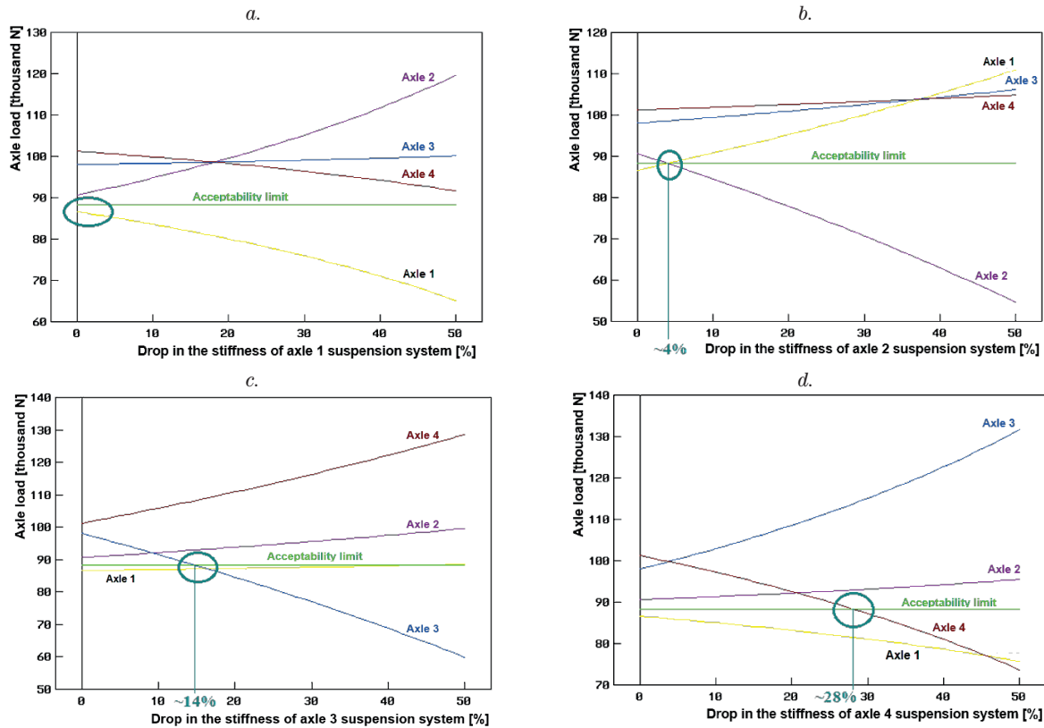
Figure 10 Motor truck. Impact of a reduction in the stiffness of suspension systems of axles 1 (a), 2 (b), 3 (c) and 4 (d) on the normal road reactions (axle loads) at pneumatic tyres of all the four vehicle axles
