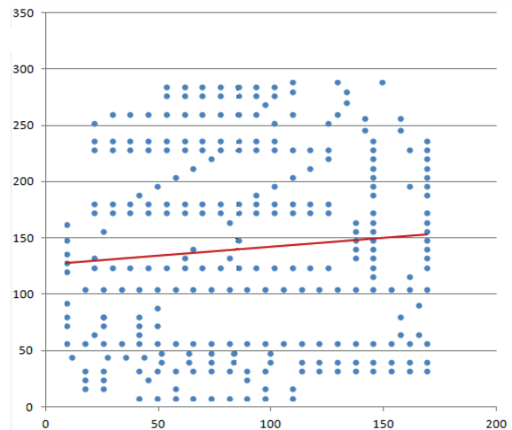
Figure 3 The regression line
